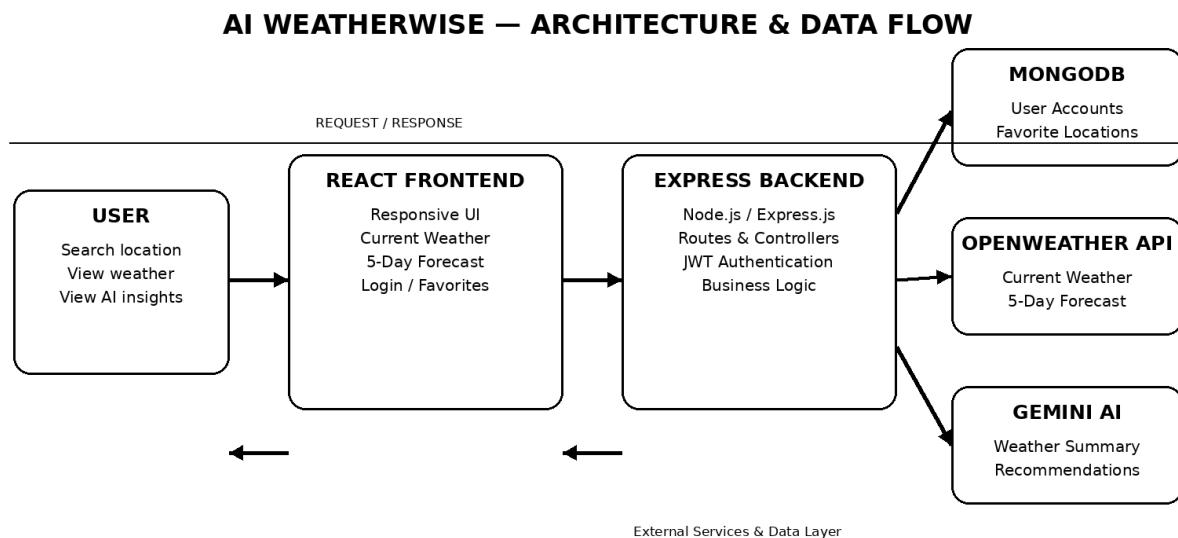
Figure 1: Architecture and data flow of the AI WeatherWise application
